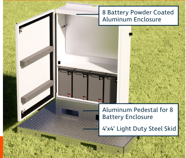
IPA-8 with PED-IPA-8 and SKID-LDS
